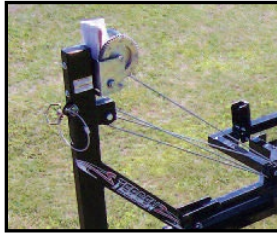
Heavy Duty Winch Stand With Brake & Double Pulley System
